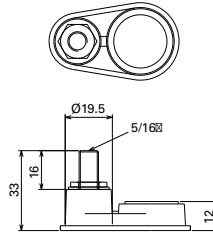
Terminal (EHPT)
